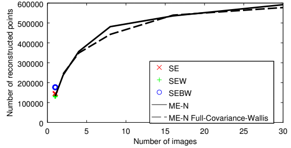
Figure 9. Wall dataset. Number of points of the dense reconstruction for different numbers of images per viewpoint
