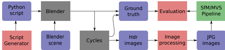
Fig. 2. Pipeline overview.
